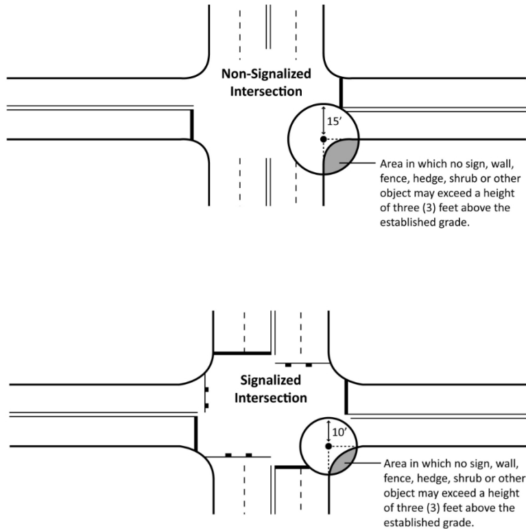
Figure 20.52-1: View Obstruction
