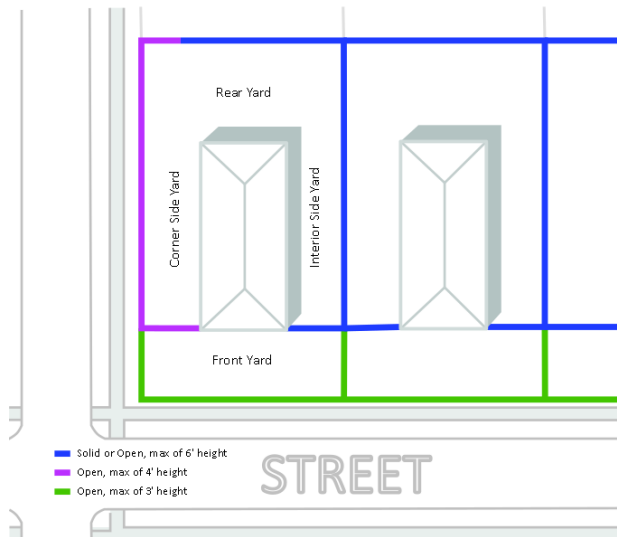
FIGURE 20.52-3: PERMITTED RESIDENTIAL FENCE LOCATION
