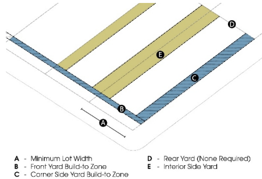
FIGURE 20.36-12: MULTI-FAMILY BUILDING
