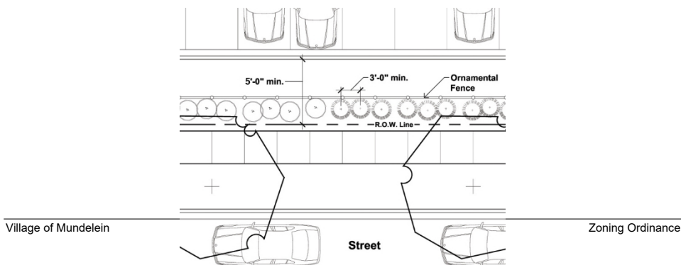
FIGURE 20.60-2: PARKING LOT PERIMETER LANDSCAPE YARD
