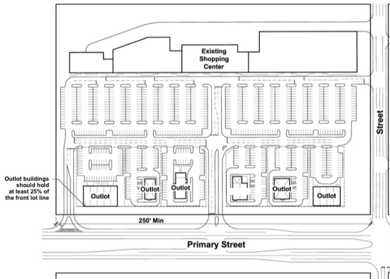
FIGURE 20.32-3: BUILDING SITING
