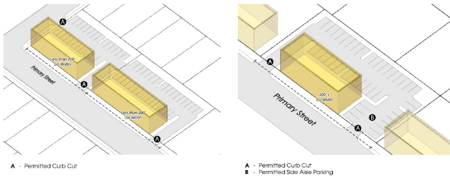
FIGURE 20.36-27C: PARKING ACCESS
