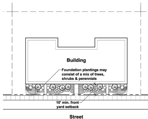
FIGURE 20.60-1: BUILDING FOUNDATION LANDSCAPE
