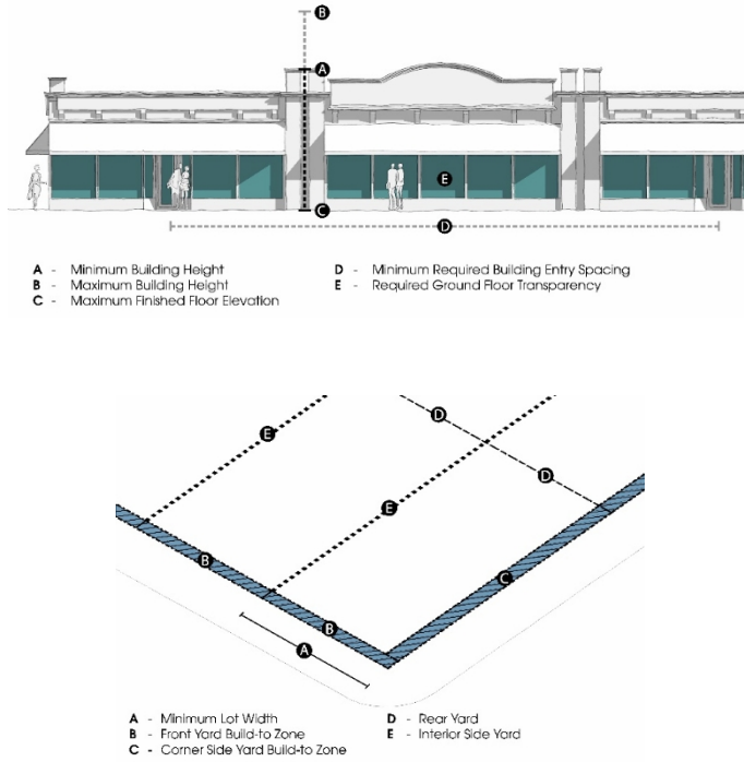
FIGURE 20.36-10: NON-RESIDENTIAL BUILDING
