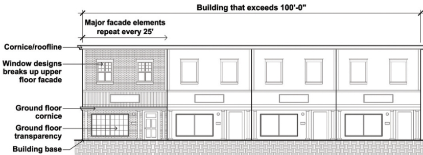
FIGURE 20.32-1: FAÇADE ARTICULATION
