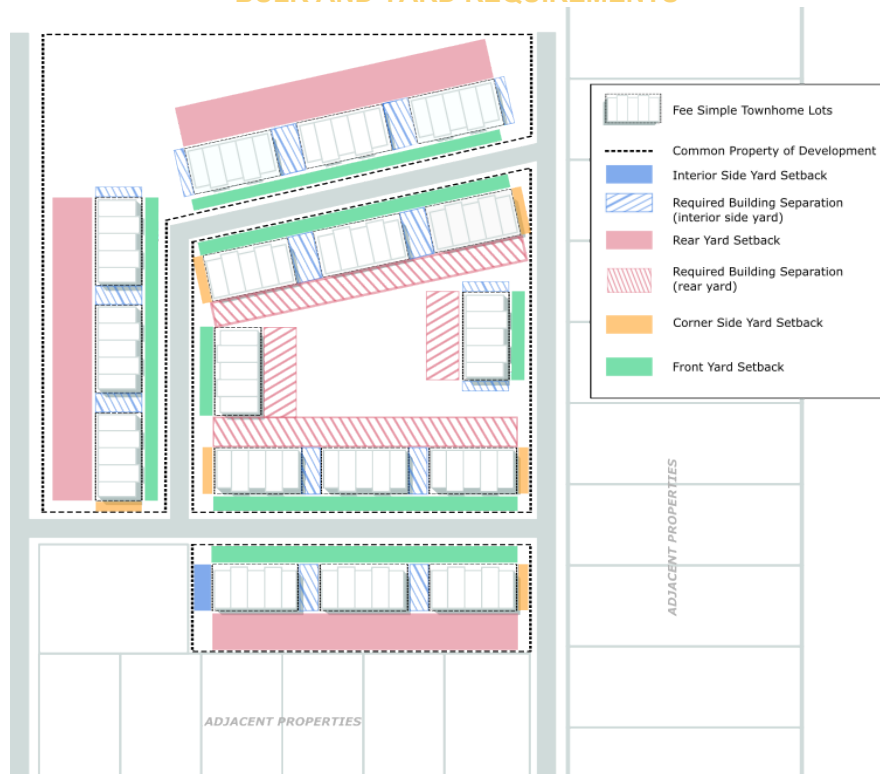
FIGURE 20.28-5: FEE SIMPLE TOWNHOUSE BULK AND YARD REQUIREMENTS TOWNHOUSE BULK AND YARD REQUIREMENTS
