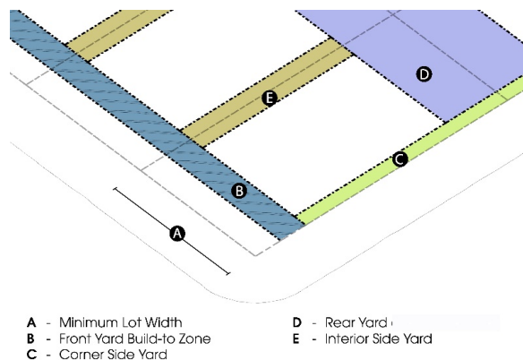
FIGURE 20.36-14: SINGLE-FAMILY, SINGLE-FAMILY ATTACHED, AND TWO-FAMILY DWELLINGS
