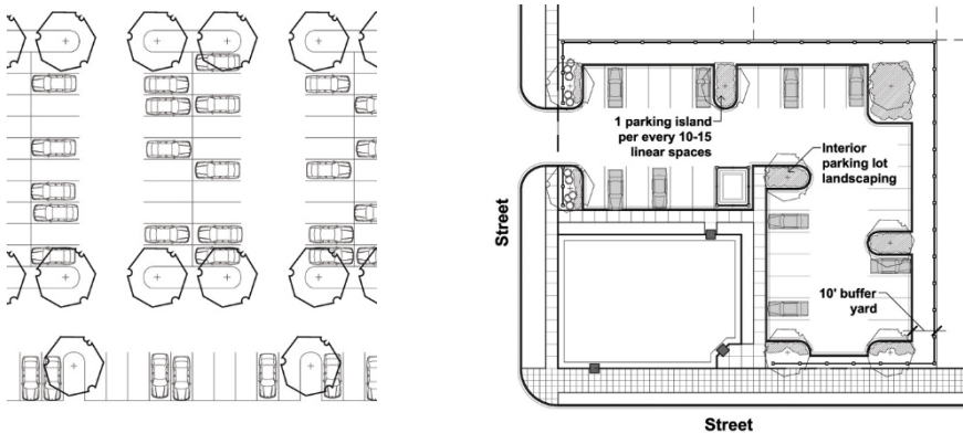
FIGURE 20.60-3: INTERIOR PARKING LOT LANDSCAPE
