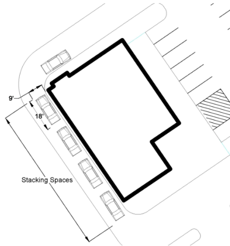
FIGURE 20.56-4: STACKING SPACES
