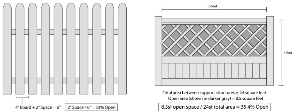
Figure 20.52-2: Examples of fences that meet the 33% openness requirement.
